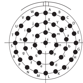
21-41/20-41 G41, 41 # 20, I
