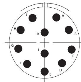
21-11 G11, 11 # 12, I
