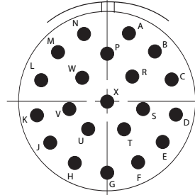
23-21/22-21 H21, 21 # 16, II
