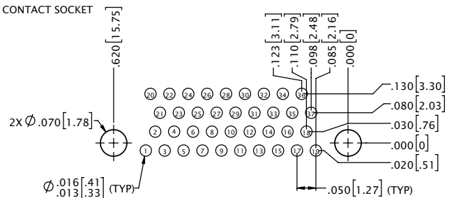
37 CONTACT SOCKET
