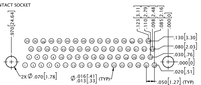
65 CONTACT SOCKET
