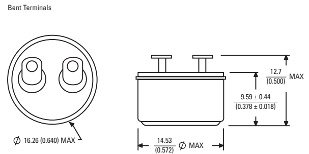
Bent Terminals
